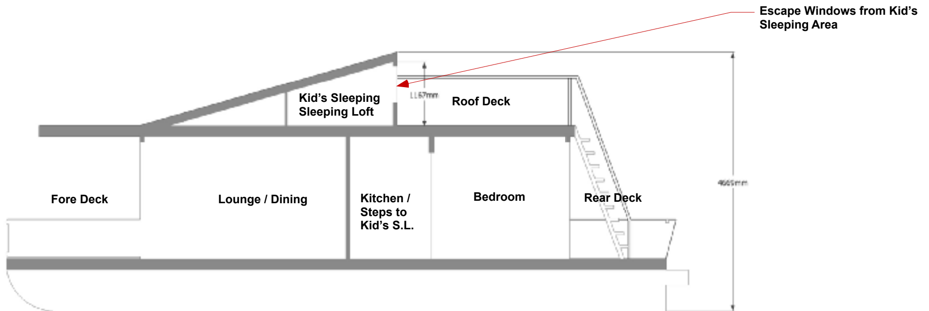
SECTION
