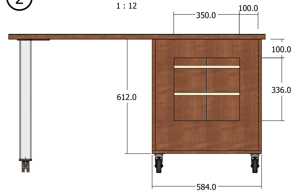
④ Elevation Arriere 1 : 12
