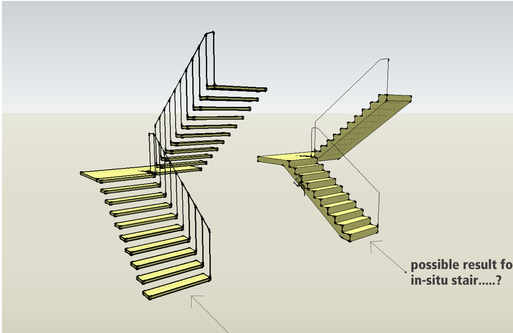
stairmaker plugin - u-shape
