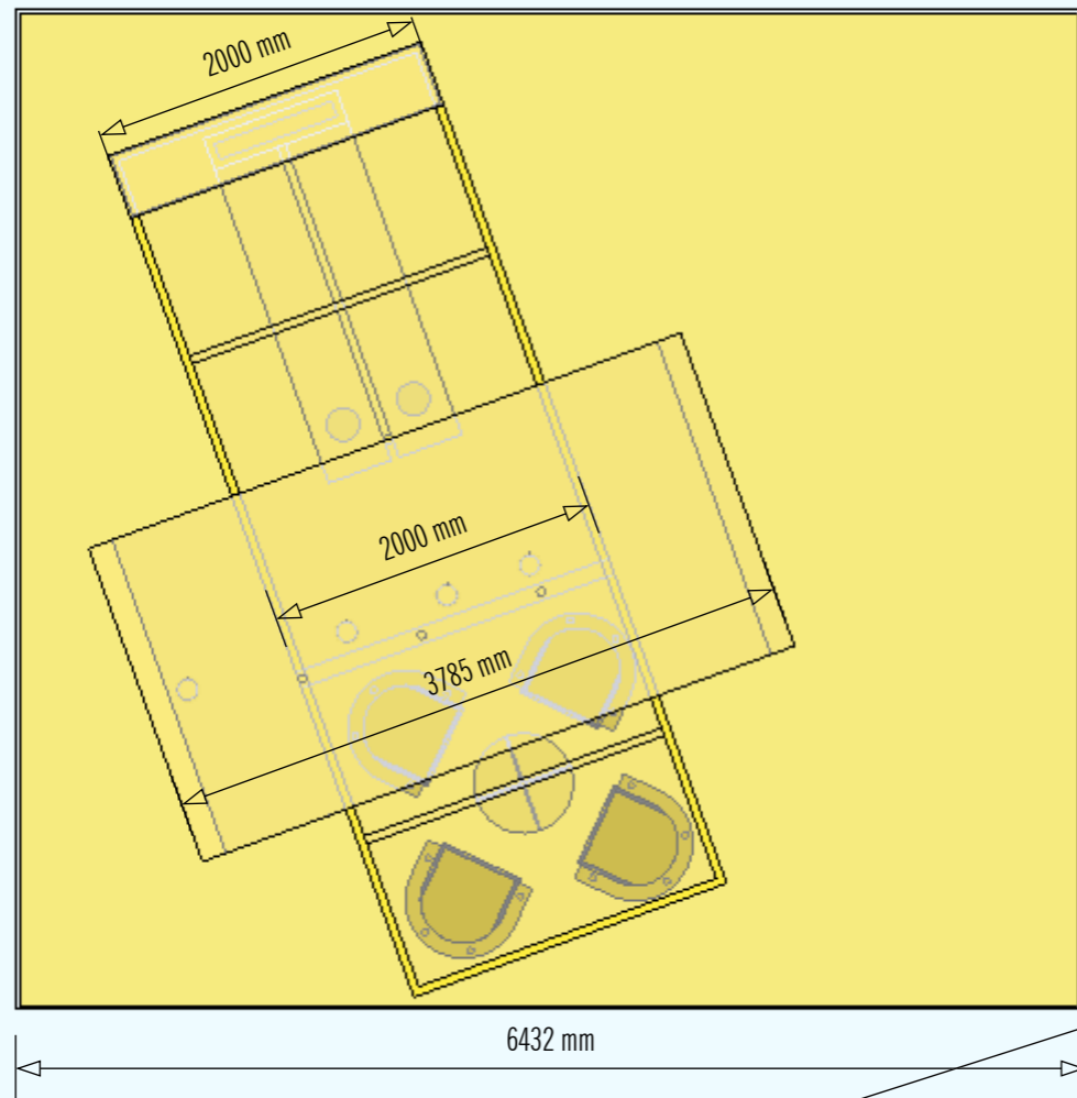
PLAN VIEW
