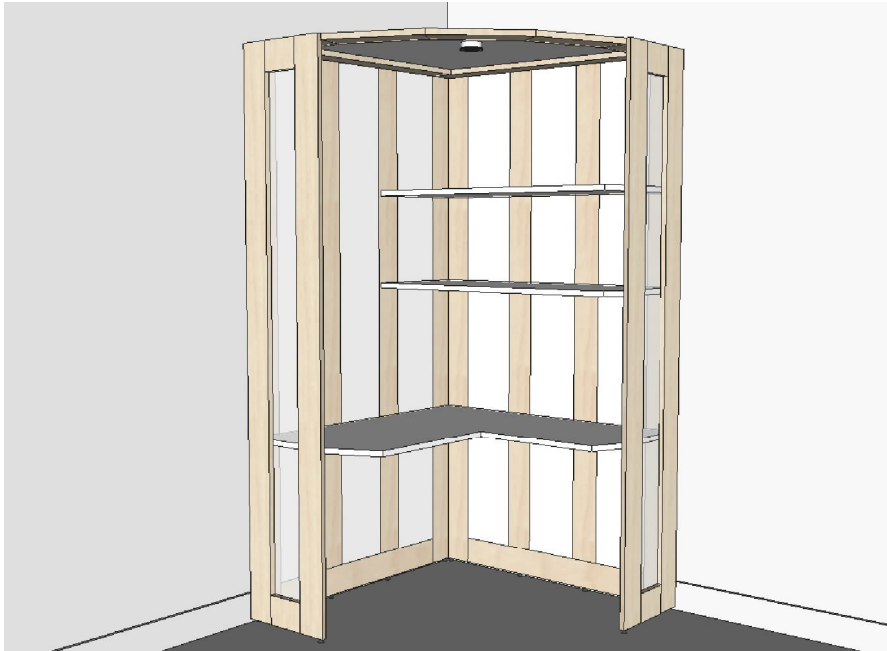
09. Work top fitted (500mm and 425mm widths)
