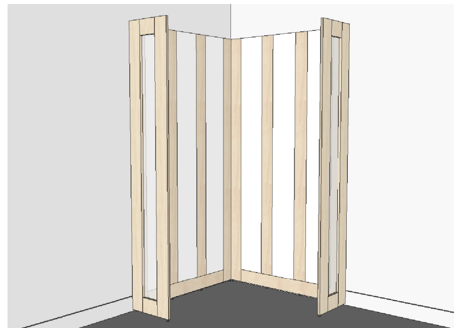
04. Left Side Front Panel (5 Pieces & 1 Leveler)
