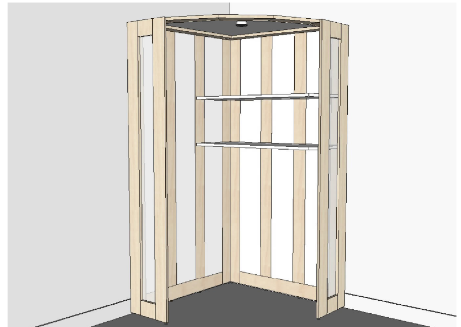
08. Two Shelves fitted (Optional L-Sheves available)
