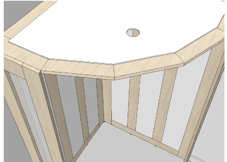
06. Top Ceiling with hole for Down Lighter (1 Piece)
