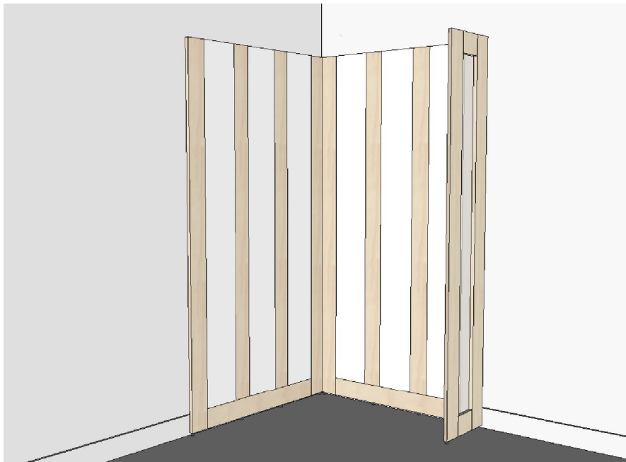
03. Right Side Front Panel (5 Pieces & 1 Leveler)
