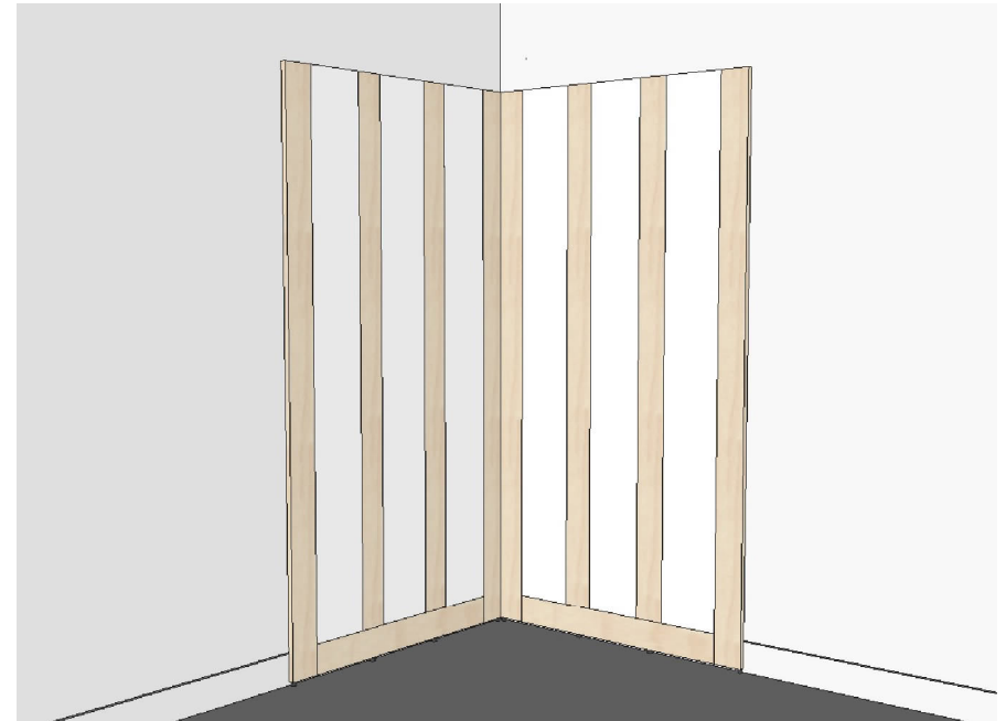
02. Right Side Rear Panel (8 Pieces & 3 Levelers)
